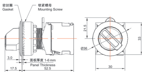
纯平短手柄 Recessed Short Handle
